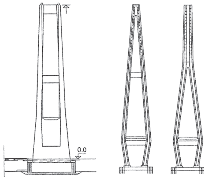
Pylons of cable-supported bridges
