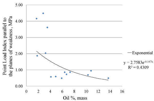
Fig. 12. Correlation between PLTI parallel to the planes of weakness and oil content (drill hole 2).
