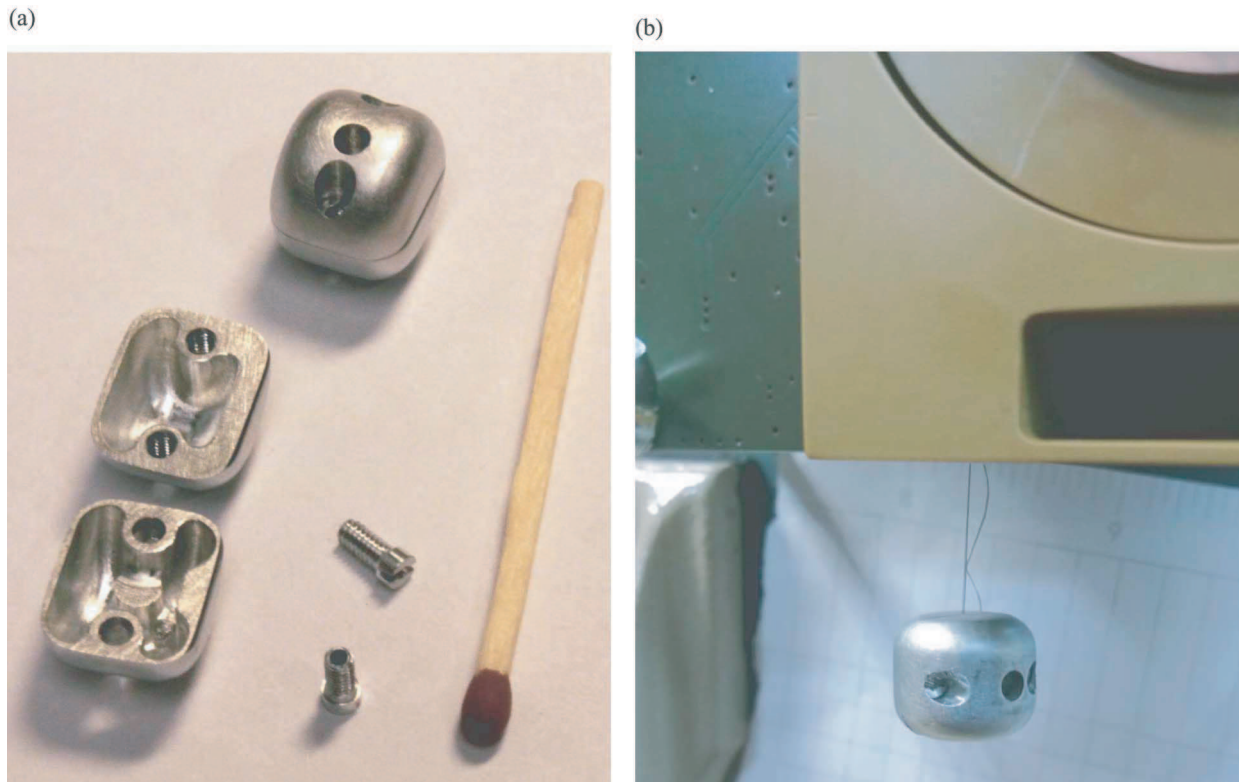
Fig. 9. (a) Assembled and stripped down view of the end mass. (b) End mass hanging from the tether during PL assembly. Tether enhanced digitally for visibility. Notice the middle hole for the launch lock pin.
