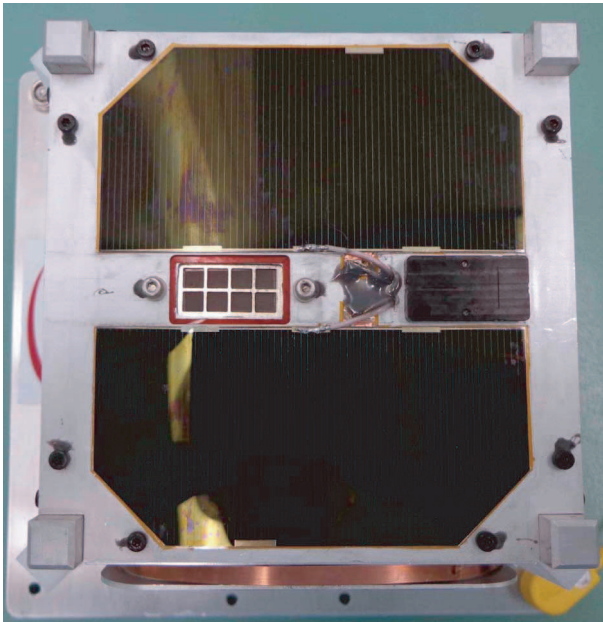
Fig. 16. Electron gun attached on the satellite side panel.
