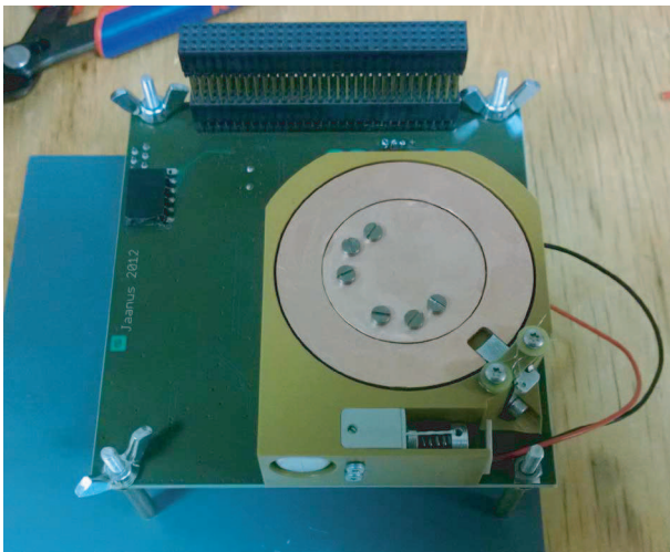
Fig. 11. Motor board fully assembled.
