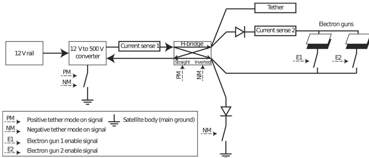
Fig. 13. Schematic presentation of the high-voltage supply.
