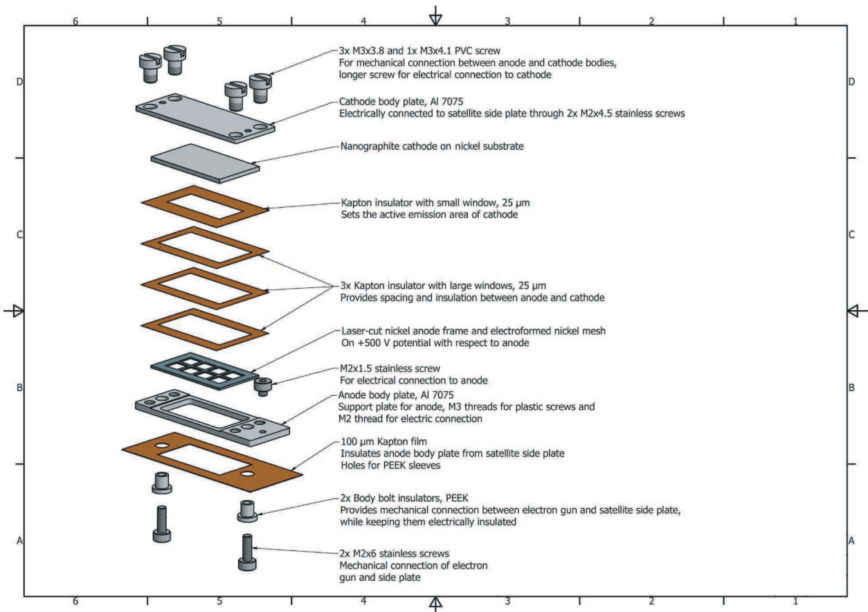
Fig. 14. Exploded view of the electron gun.
