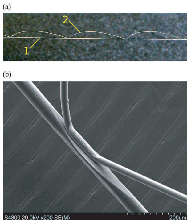
Fig. 3. Two-filament Heytether. (a) Photograph of the tether. Labels: (1) basewire, (2) loop wire. Distance between bonds is 10 mm. (b) Scanning Electron Microscope (SEM) image of an ultrasonic wire-to-wire bond.
