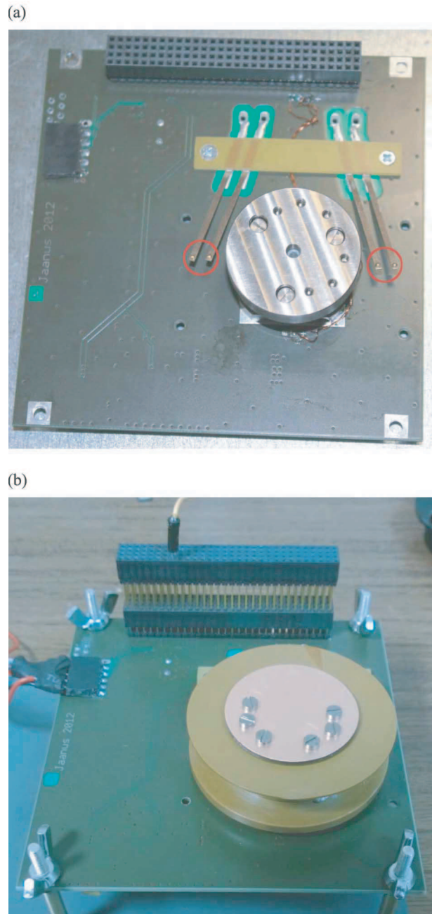
Fig. 6. Different stages of motor board assembly. (a) Reel motor attached on the circuit board. Shown circled are the four slip ring contacts. (b) Tether reel attached on the motor.
