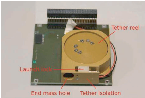
Fig. 5. Motor board partly assembled. The two electric wires on the right are used for releasing the launch lock. They were not connected to their terminals on the circuit board at the time of this photograph.
