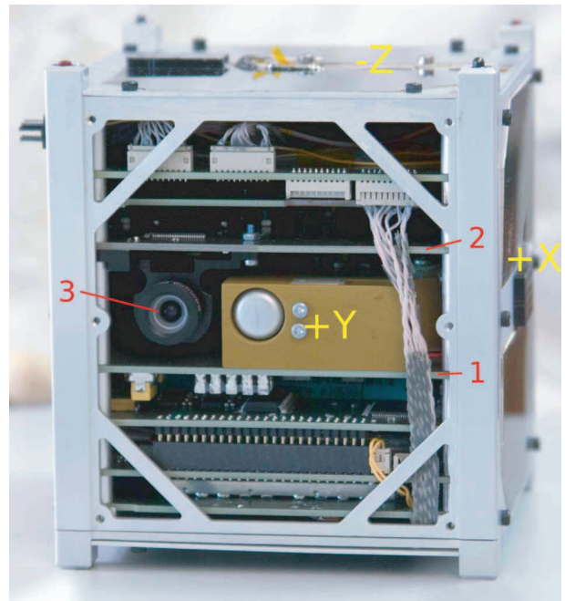
Fig. 2. Assembled satellite with side panels removed. Labels: (1) motor board, (2) HV board, (3) onboard camera. The yellow labels denote the directions of the X, Y, and Z axes of the satellite’s coordinate system.
