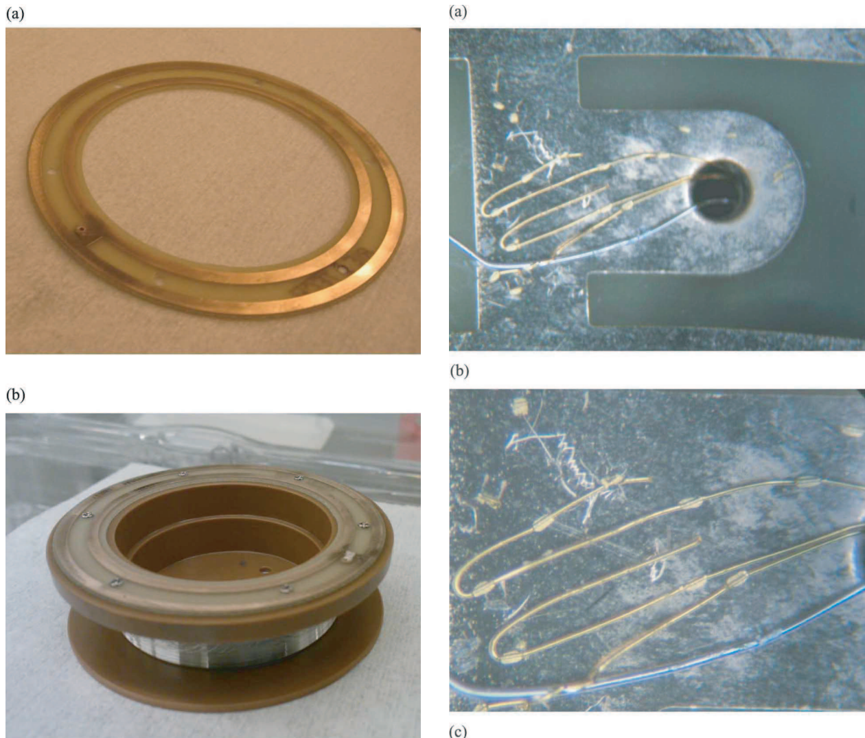
Fig. 7. Slip ring. (a) Bare slip ring. (b) Slip ring attached on the reel, tether bonded, and reeled.
