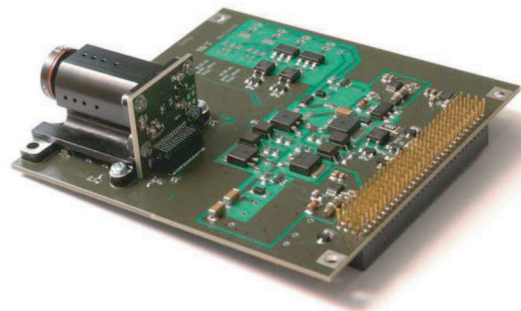
Fig. 12. High-voltage board. The large black block is the onboard camera.
