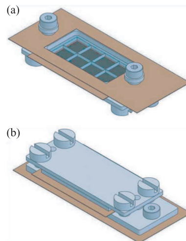
Fig. 15. Two views of the assembled electron gun. “Top” is the direction of the emitted electron beam. (a) Top view. (b) Bottom view.
