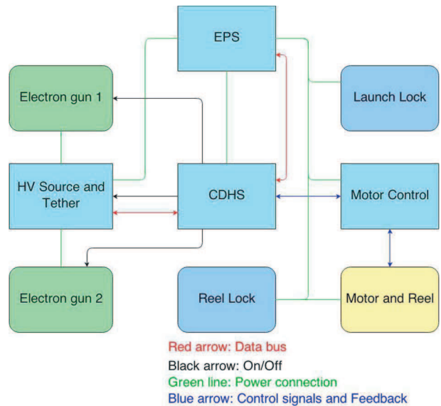
Fig. 1. Block diagram depicting the data and power interactions between PL parts, CDHS, and EPS.
