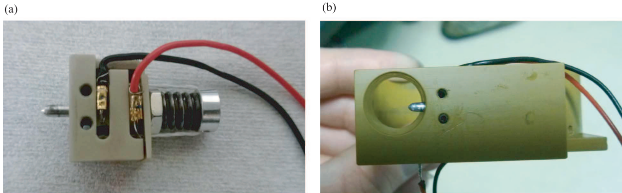
Fig. 10. (a) Launch lock, loaded. (b) Launch lock placed at its position in tether isolation. Notice the pin entering the end mass compartment.
